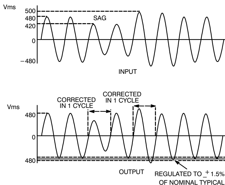
REGULATED SYSTEM RESPONSE
